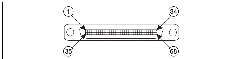
Figure 1. IMAQ 6804 68-pin VHDCI Connector
