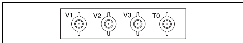
Figure 2. IMAQ A6804 BNC Connectors
